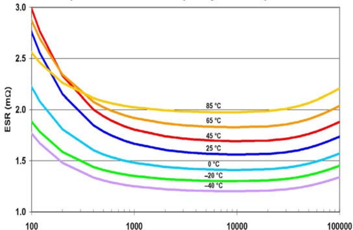
230 \mu\text{F} 1000 V ESR vs Frequency and Temperature
