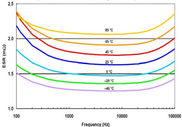
490 \mu\text{F} 800 V ESR vs Frequency and Temperature
