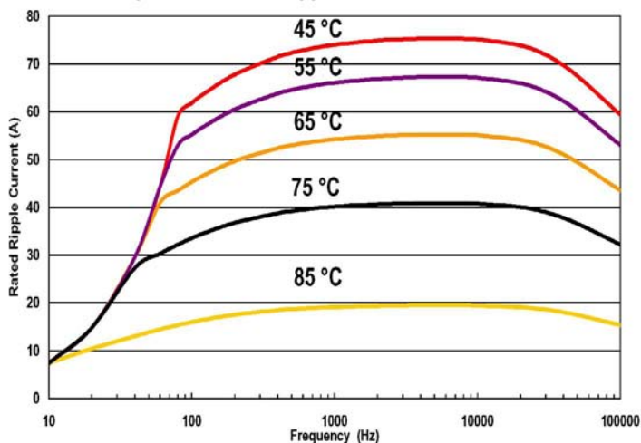
490 \mu\text{F} 800 V Rated Ripple Current, Still Air, 5 kh Life
