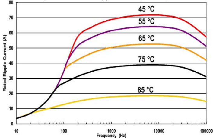
230 \mu\text{F} 1000 V Rated Ripple Current, Still Air, 5kh Life
