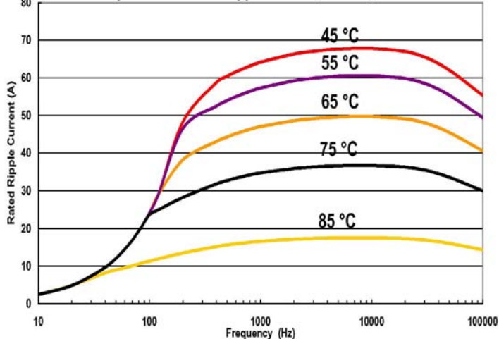
160 \mu\text{F} 1200 V Rated Ripple Current, Still Air, 5kh Life
