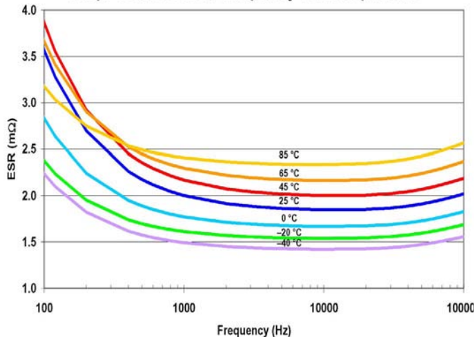
160 \mu\text{F} 1200 V ESR vs Frequency and Temperature
